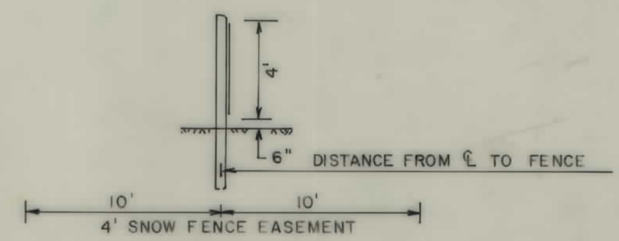
SECTION B - B 4 VERTICAL SLAT CANADIAN TYPE SNOW FENCE
