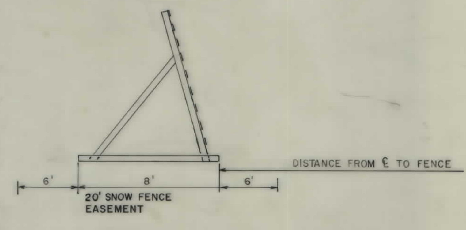
SECTION A - A 8' WYOMING TYPE SNOW FENCE
