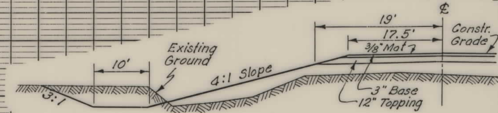
TYPICAL SECTION - CHANNEL CHANGE STA. 22+30 TO 35+40
