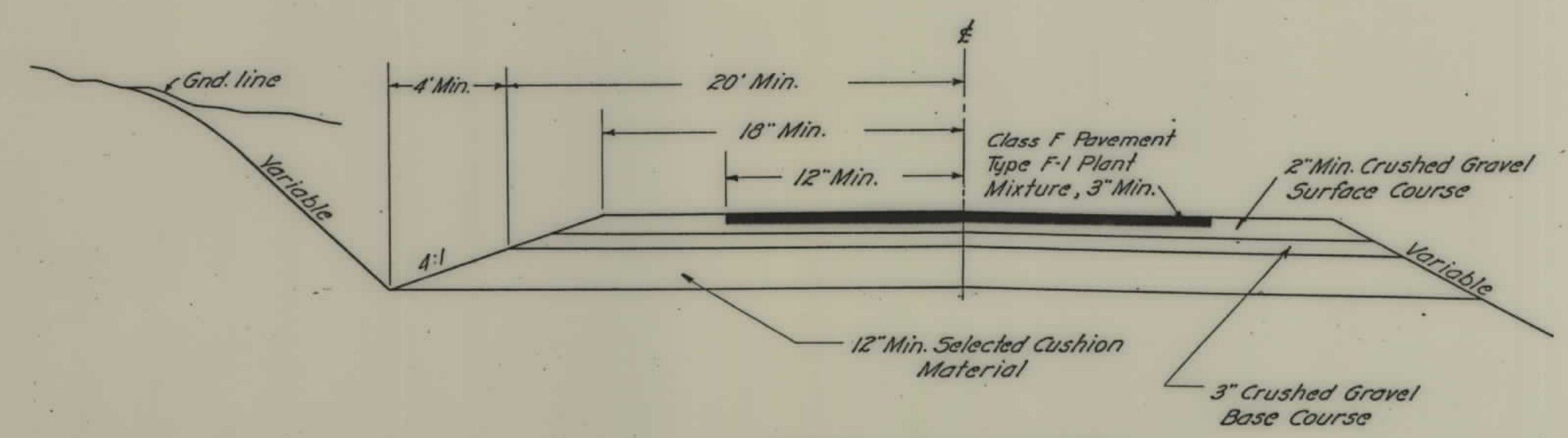
TYPICAL SECTION
