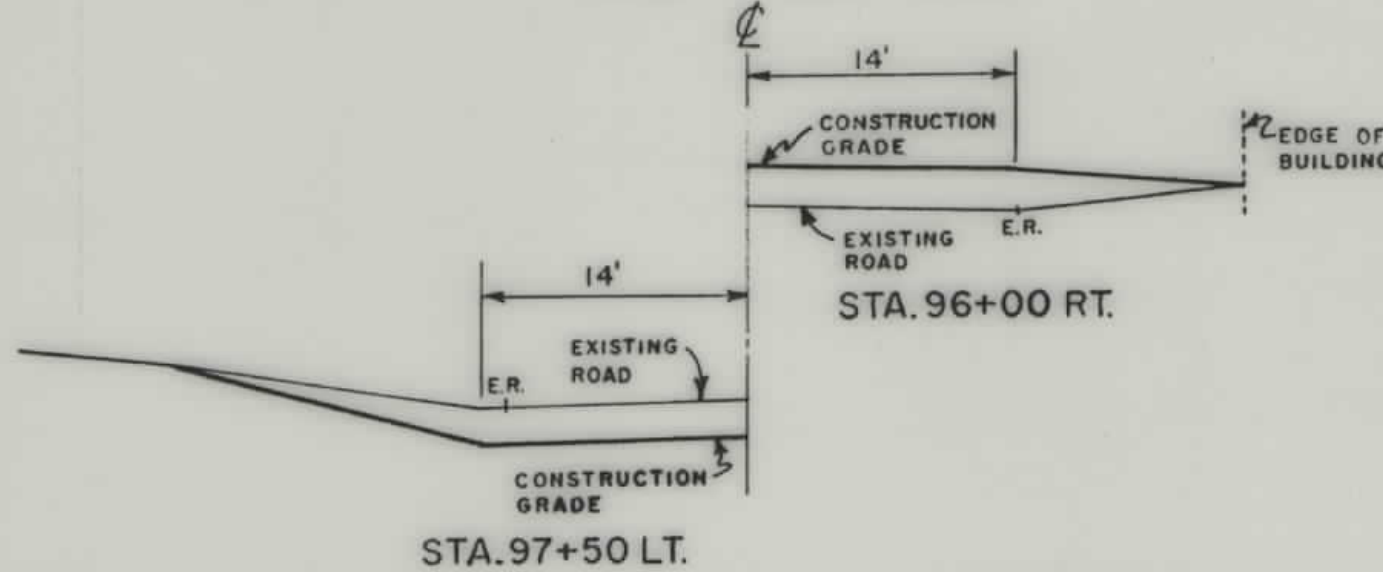
TYPICAL SECTION STA.94+00 to STA.101+25 HALF SECTIONS
